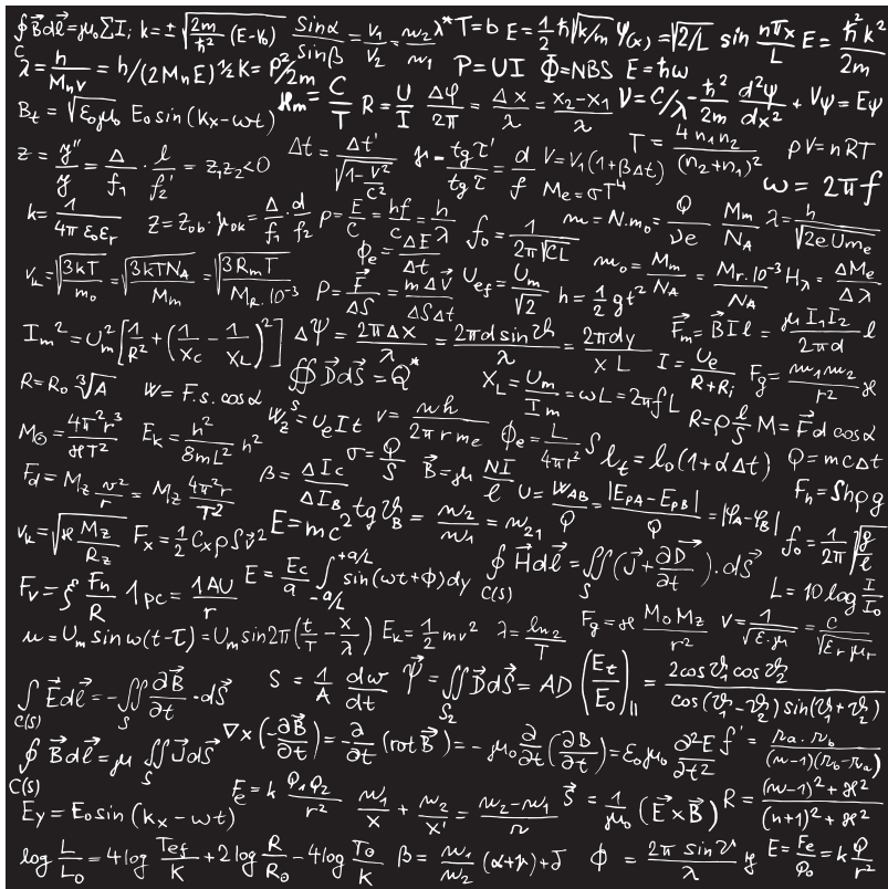
Figure 7.2 A non-physicist's view of a physics problem
