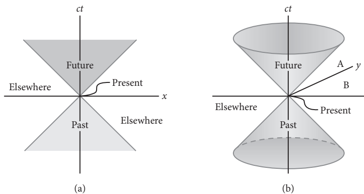
Figure 7.11 Special Relativity
