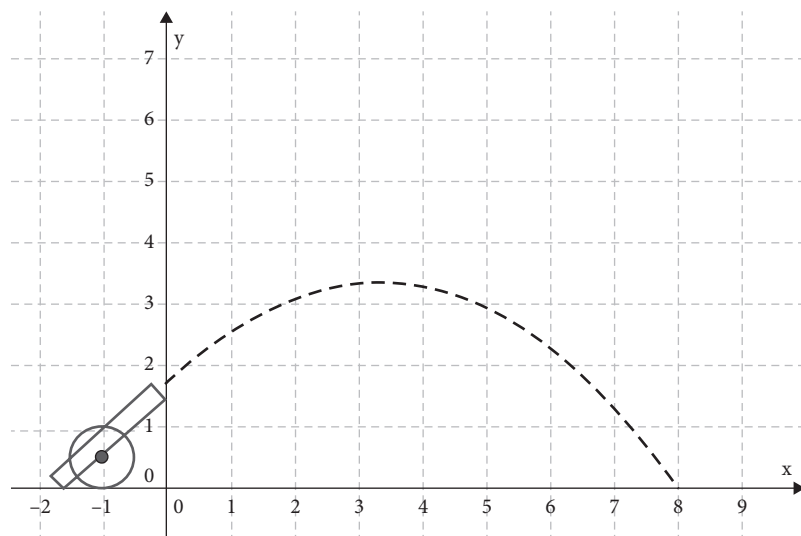
Figure 7.5 The motion of a cannonball
