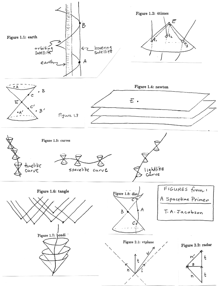
QAQ1 Figure 7.1 Teaching notes from a primer on relativity Source: © Theodore Jacobson. Reproduced with permission.
